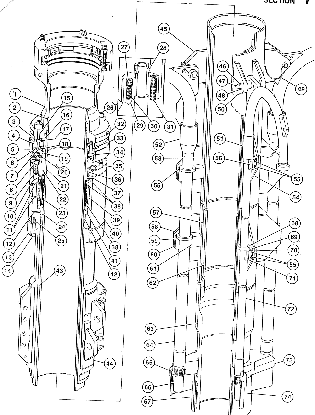
Upper Housing and Seal Subassemblies And Outer Barrel Weldment
