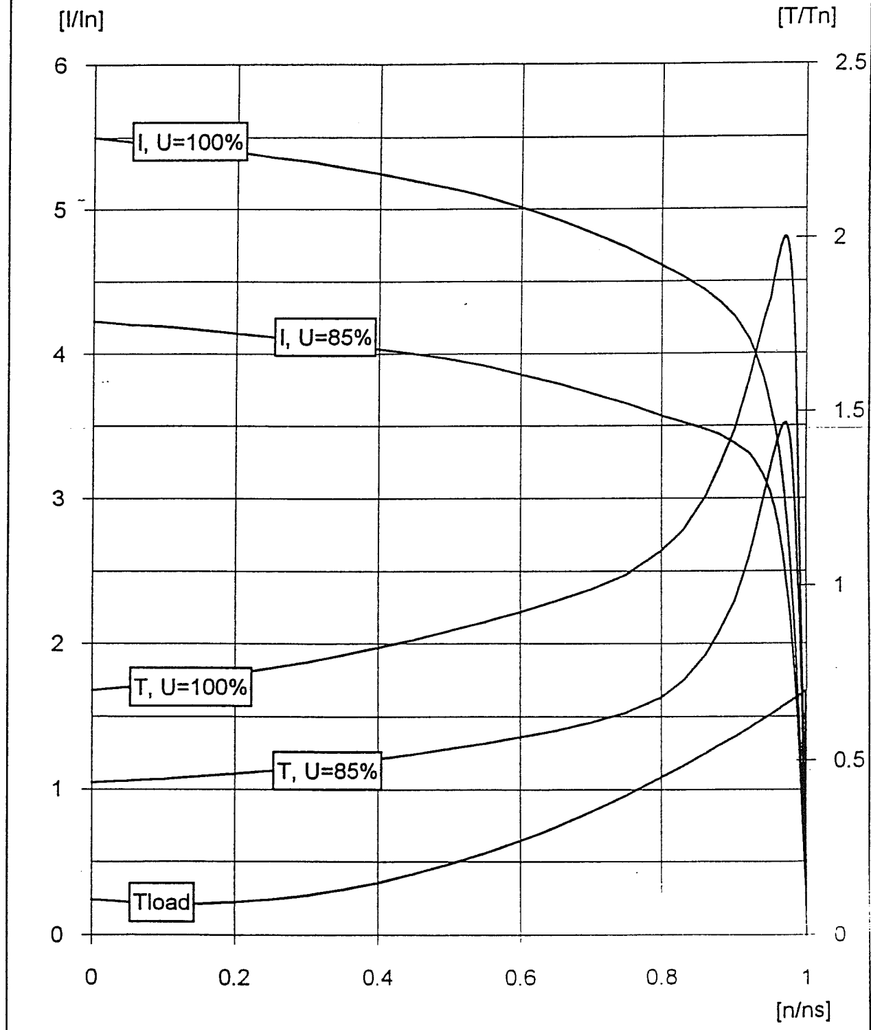
TORQUE AND CURRENT IN FUNCTION OF SPEED
