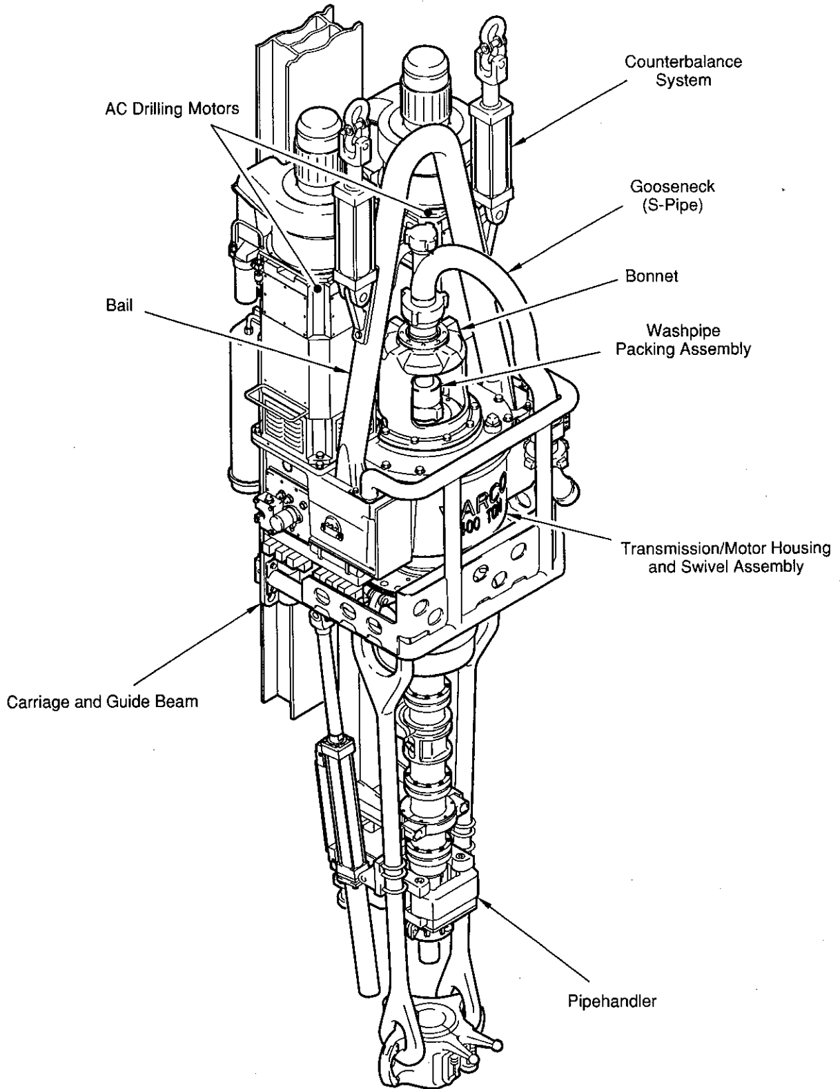
Figure 1-1. Typical TDS-9S
