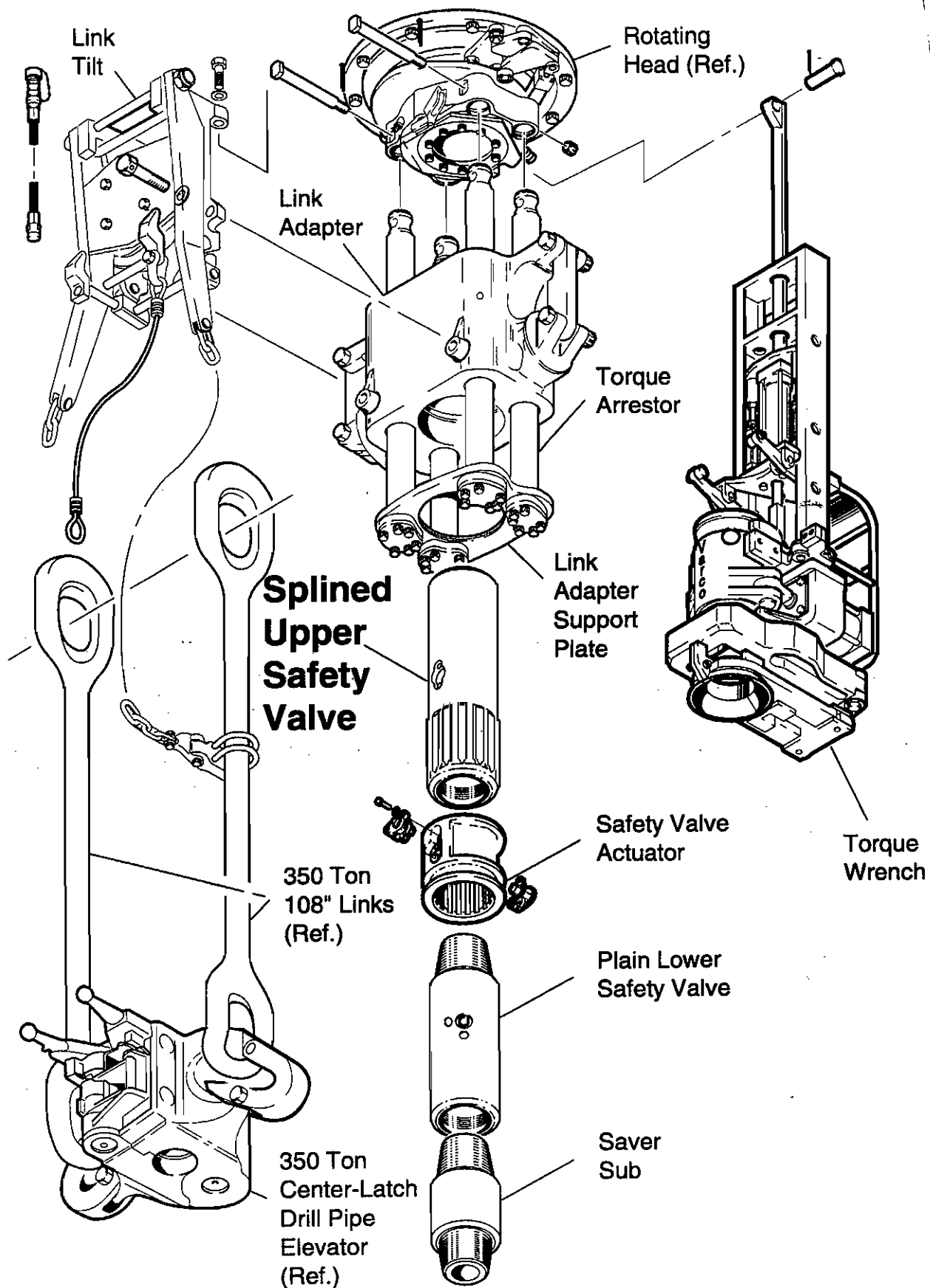
Figure 2. Typical Safety Valve in Relation to Other TDS Assemblies (PH-85, PH-60d)
