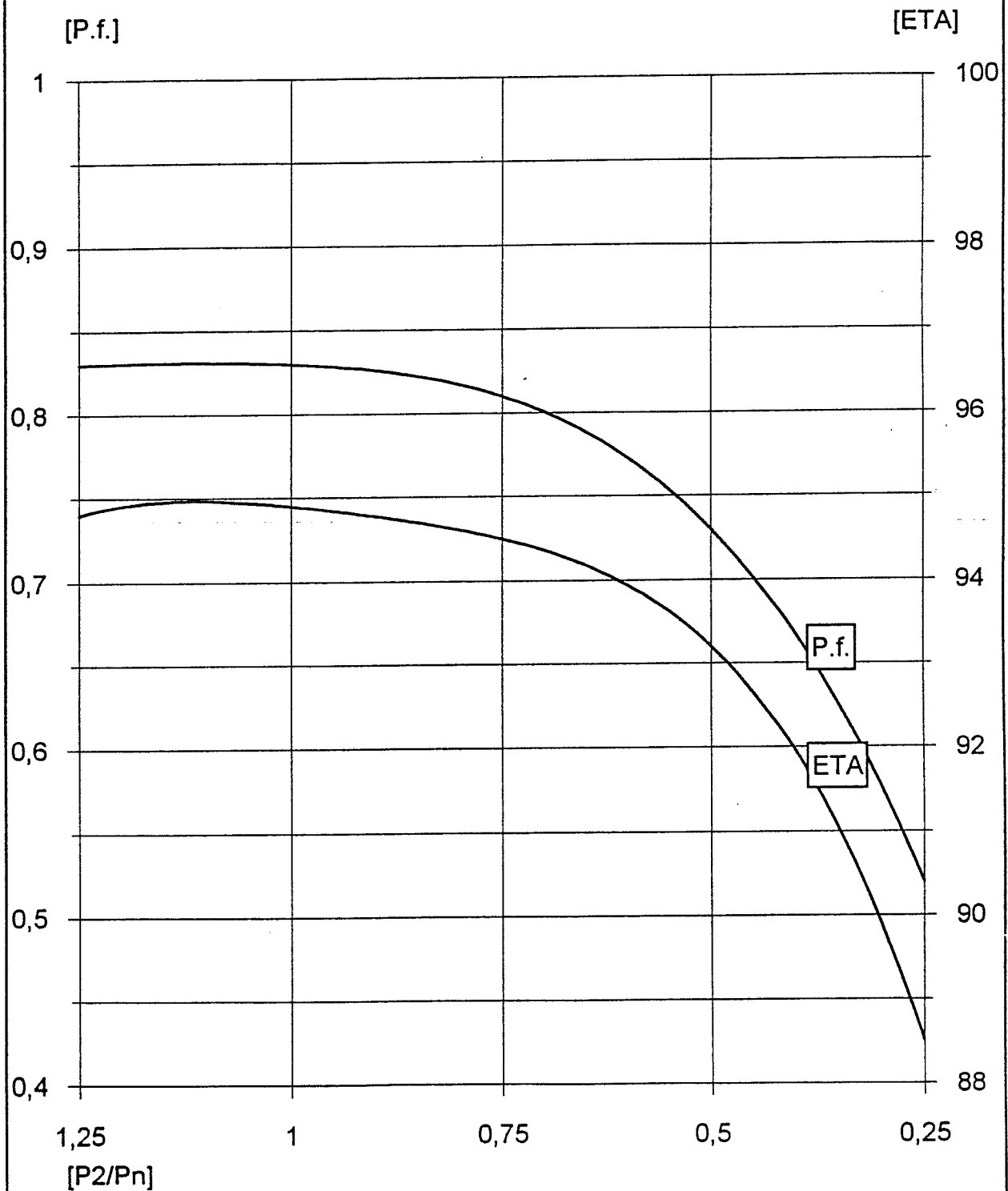
POWER FACTOR AND EFFICIENCY IN FUNCTION OF POWER
